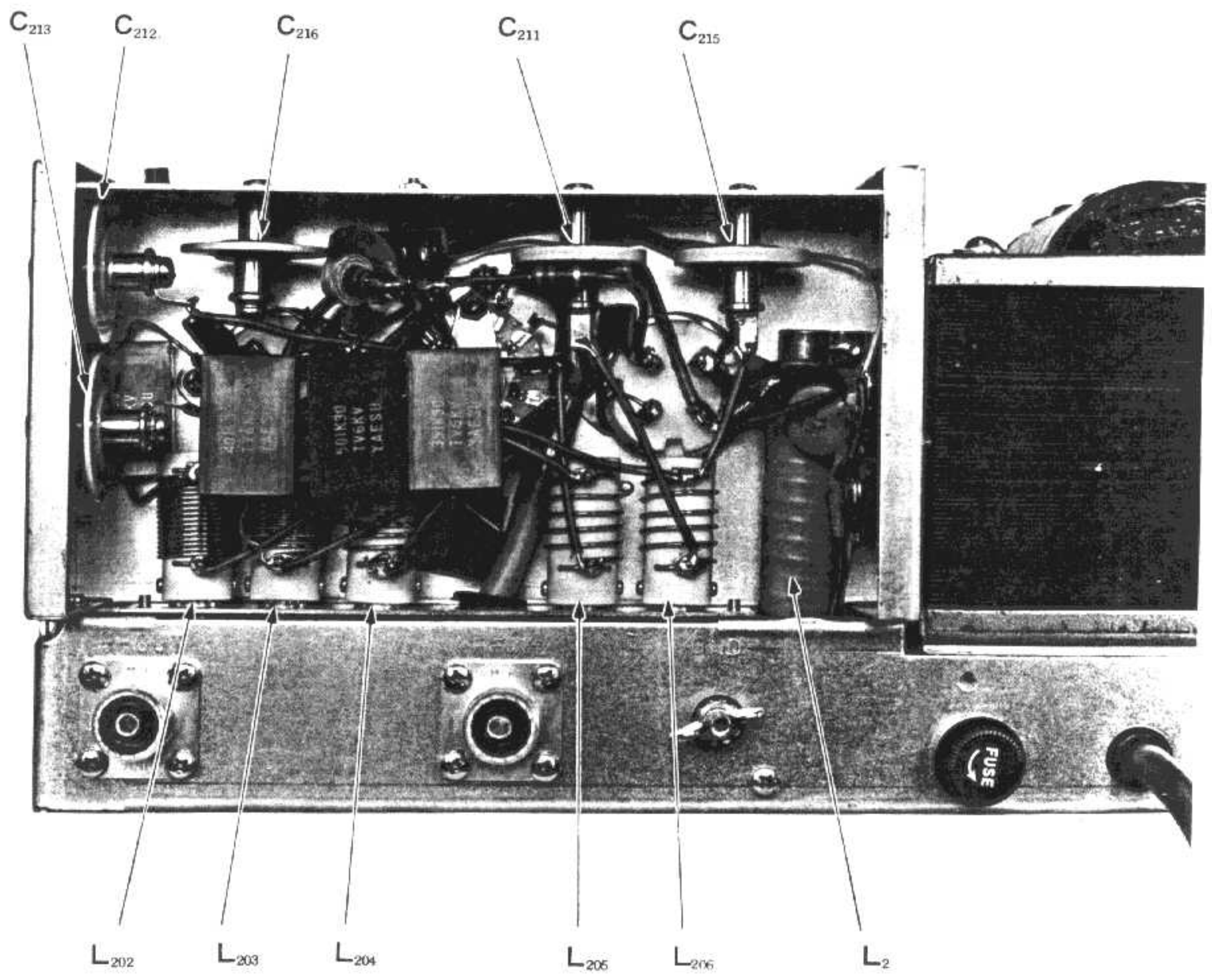
INPUT TUNING CIRCUIT
